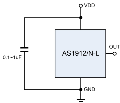
Figure 1, Typical Application Circuit of AS1912/N-L
