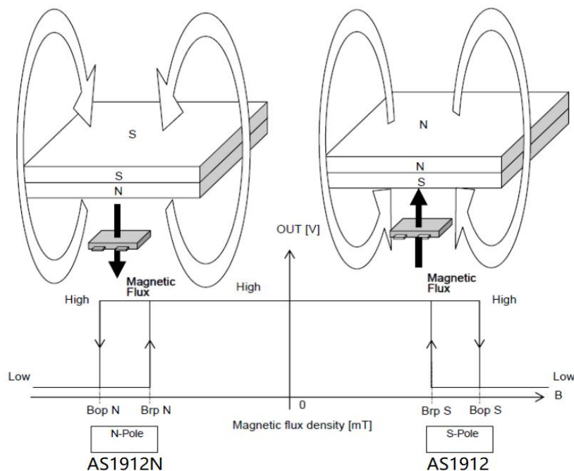
Fig 4, Magnetic Operation Characteristic of AS1912-L or AS1912N-L
