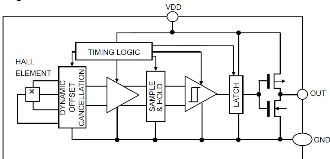
Figure 3, Block Diagram of AS1912/N-L
